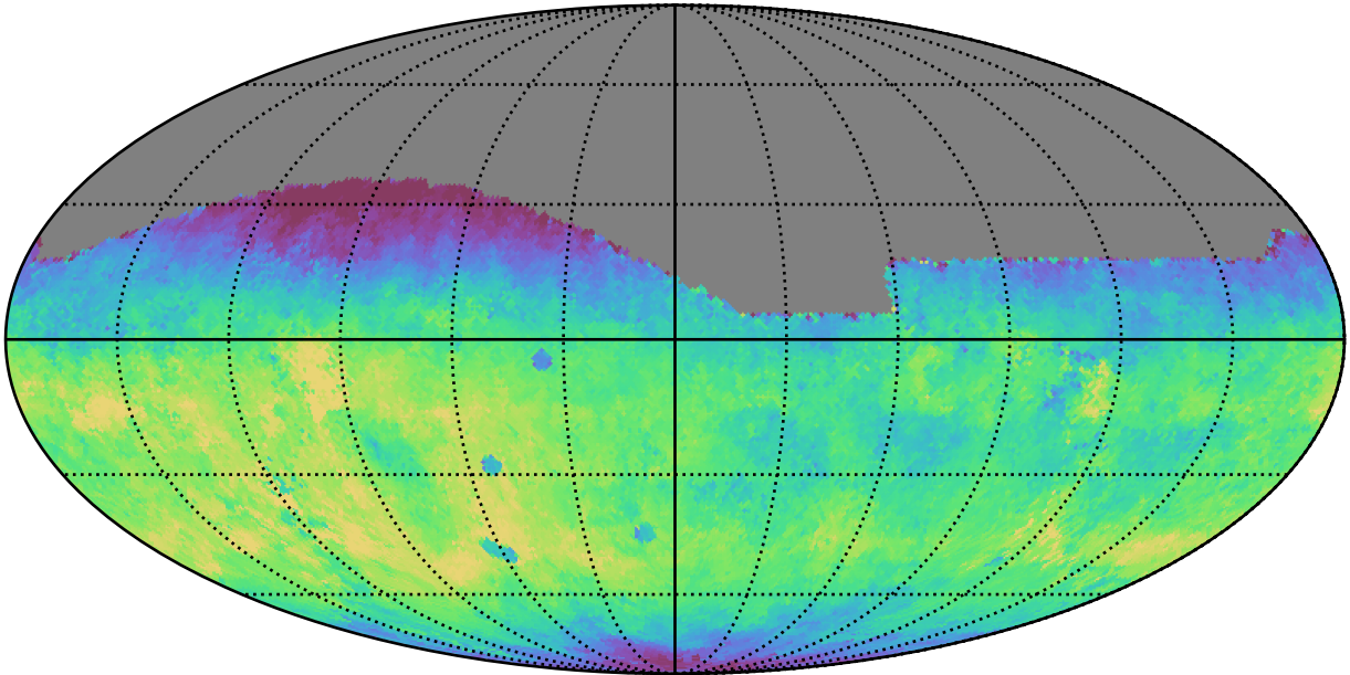
early_ss_template_fpextra2.0_v3.4_10yrs All sky g band: Median fiveSigmaDepth
