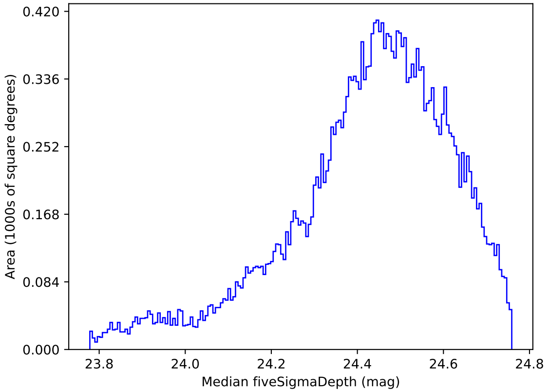
early_ss_template_fpextra2.0_v3.4_10yrs All sky g band: Median fiveSigmaDepth
