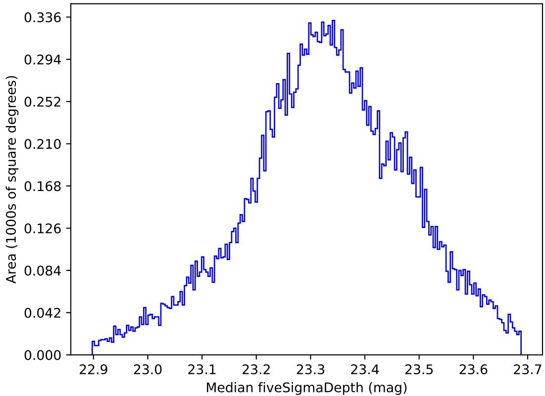
early_ss_template_fpextra2.0_v3.4_10yrs All sky all bands: Median fiveSigmaDepth
