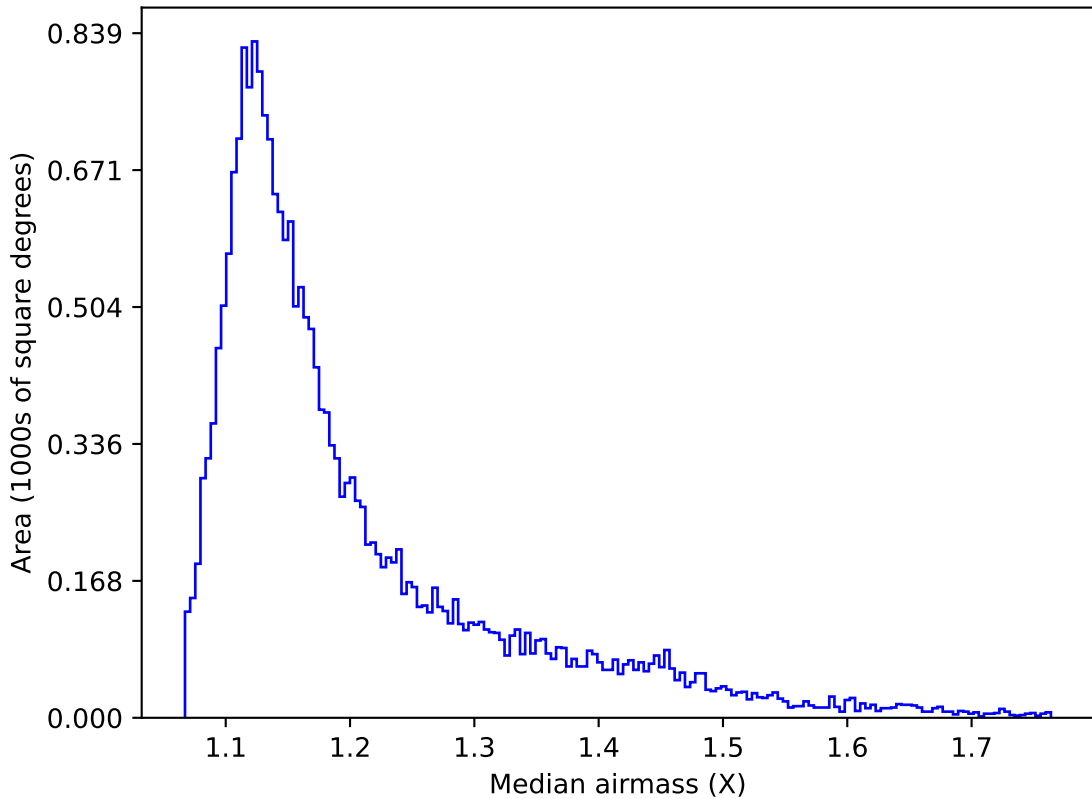
early_ss_template_fpextra2.0_v3.4_10yrs Yr 1 y band: Median airmass
