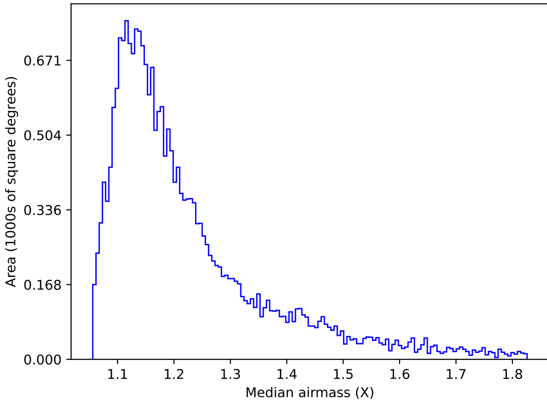
early_ss_template_fpextra2.0_v3.4_10yrs Yr 1 u band: Median airmass
