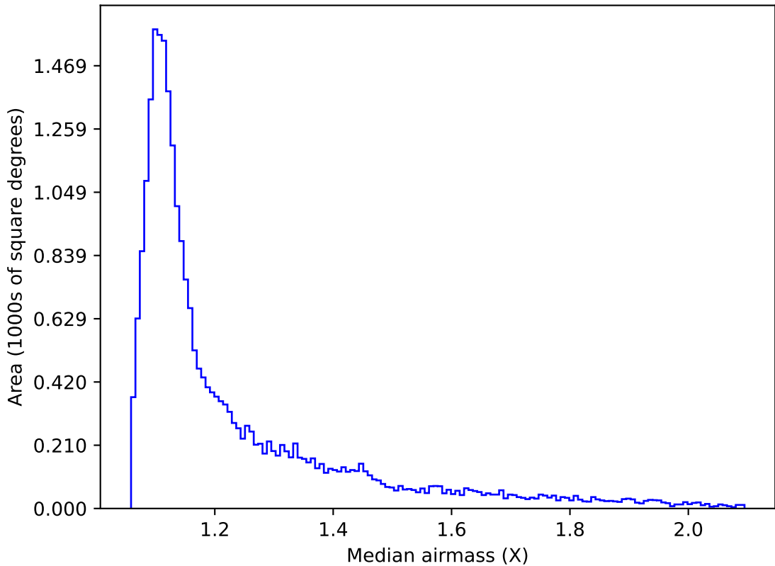
early_ss_template_fpextra2.0_v3.4_10yrs Yr 1 i band: Median airmass
