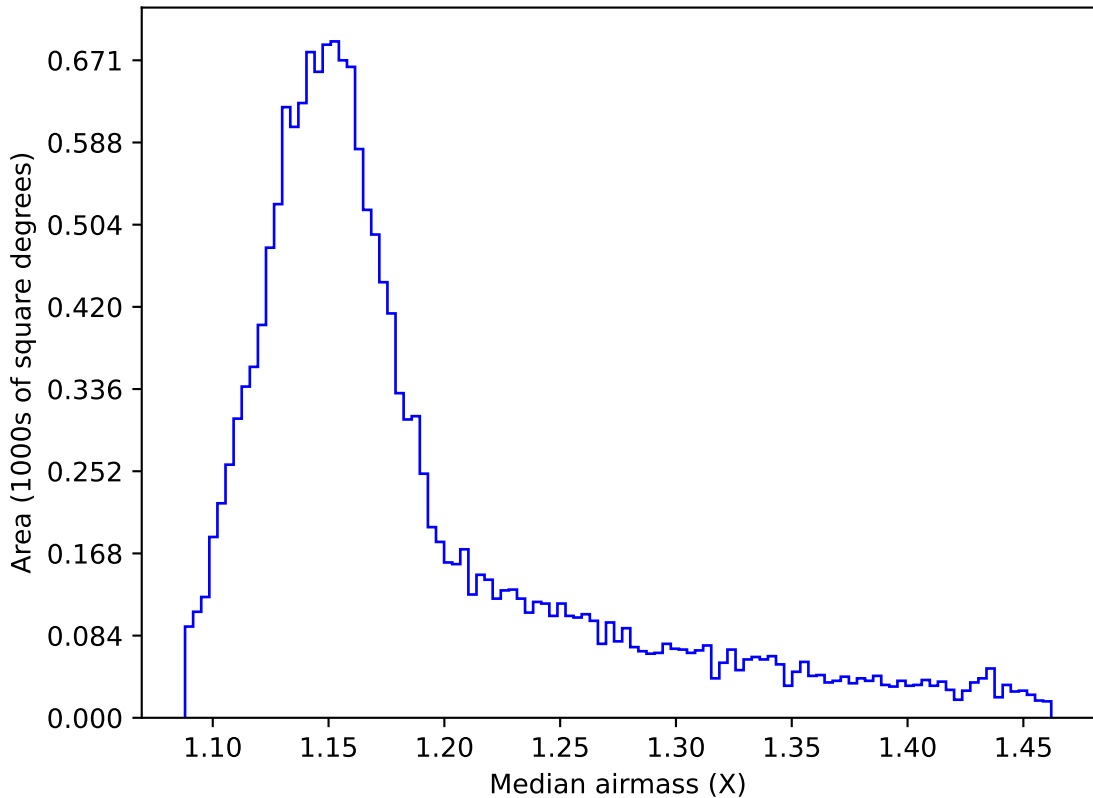
early_ss_template_fpextra2.0_v3.4_10yrs WFD z band: Median airmass
