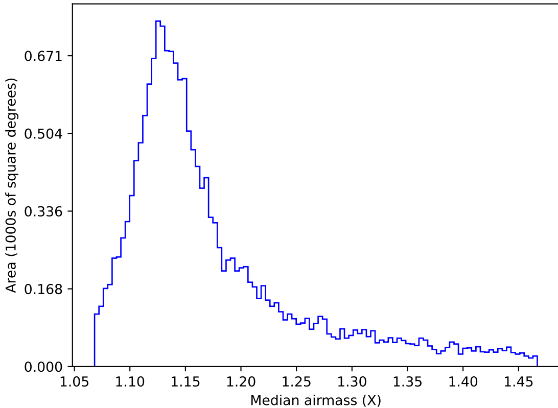
early_ss_template_fpextra2.0_v3.4_10yrs WFD u band: Median airmass
