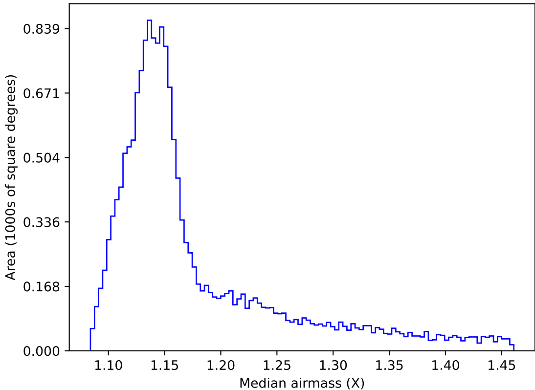
early_ss_template_fpextra2.0_v3.4_10yrs WFD all bands: Median airmass
