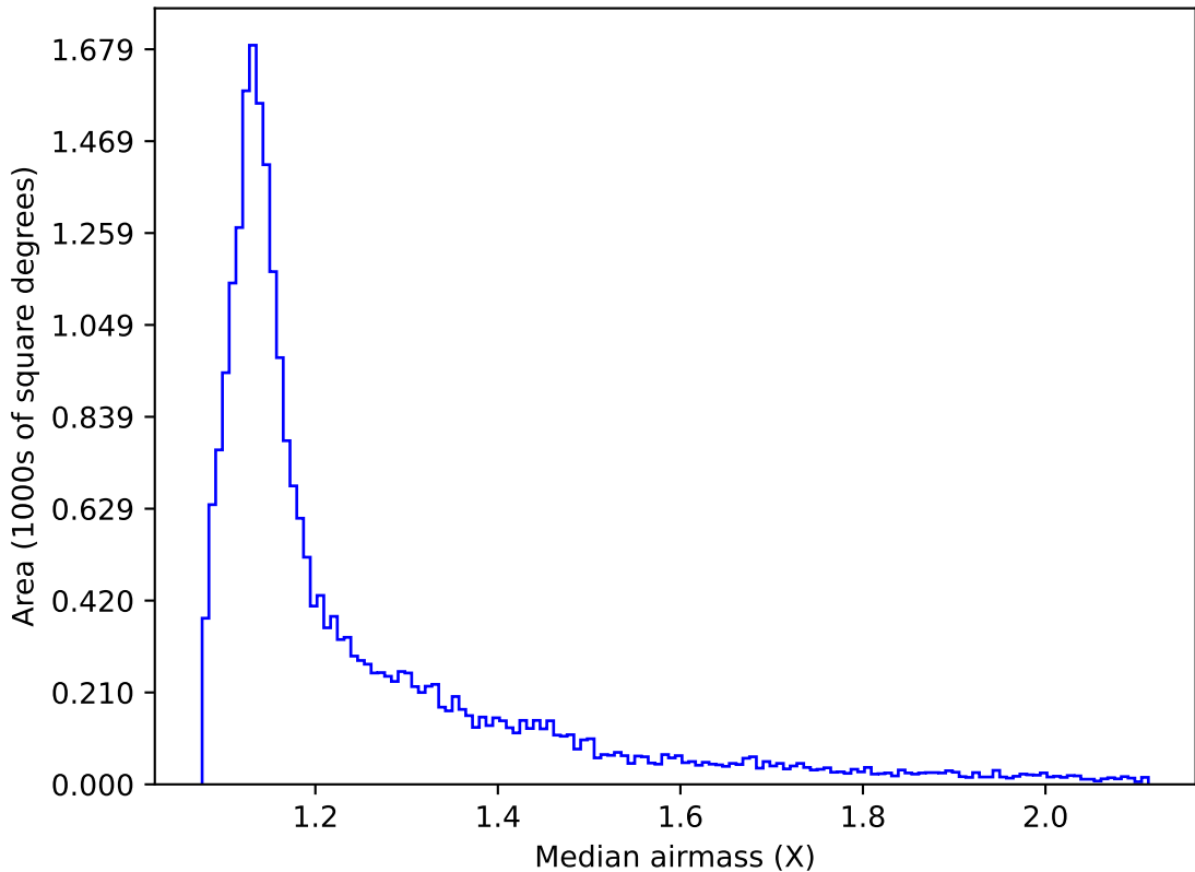
early_ss_template_fpextra2.0_v3.4_10yrs All sky g band: Median airmass
