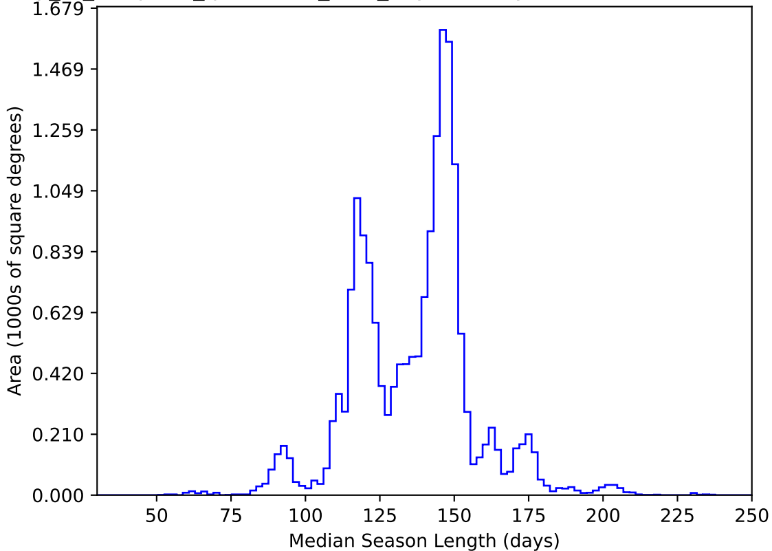
early_ss_template_fpextra2.0_v3.4_10yrs WFD y band: Median Season Length
