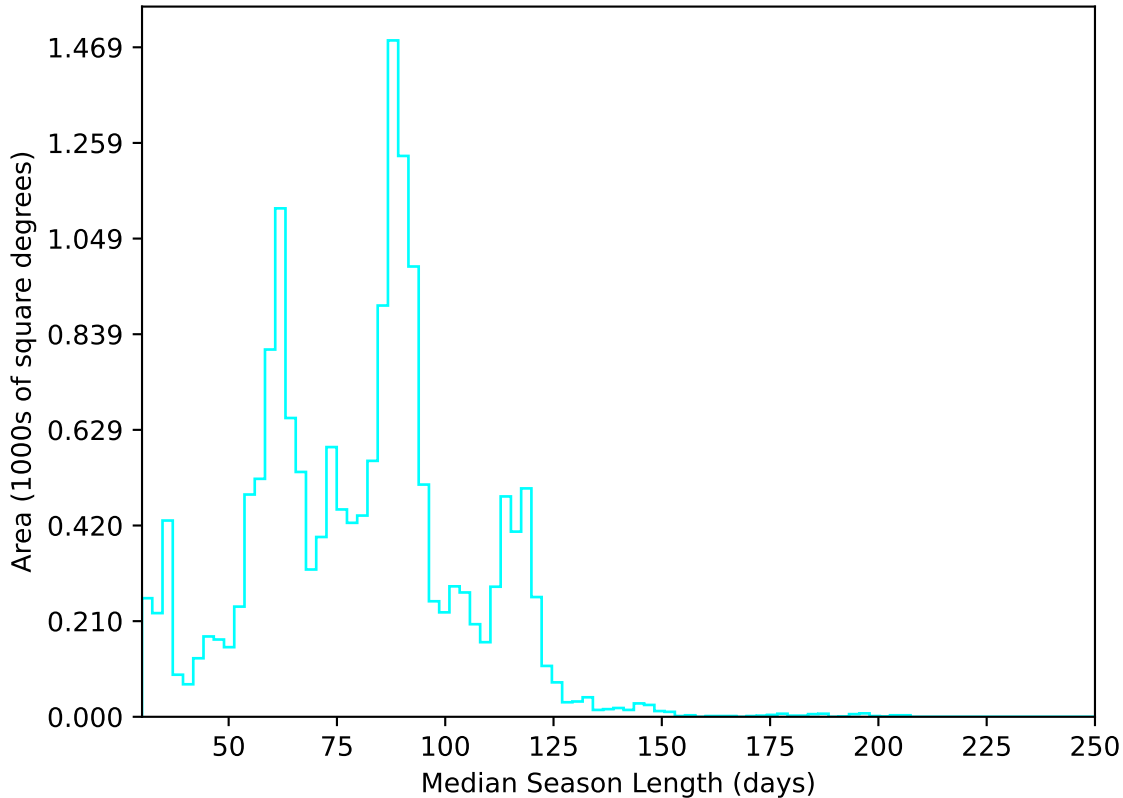
early_ss_template_fpextra2.0_v3.4_10yrs WFD u band: Median Season Length
