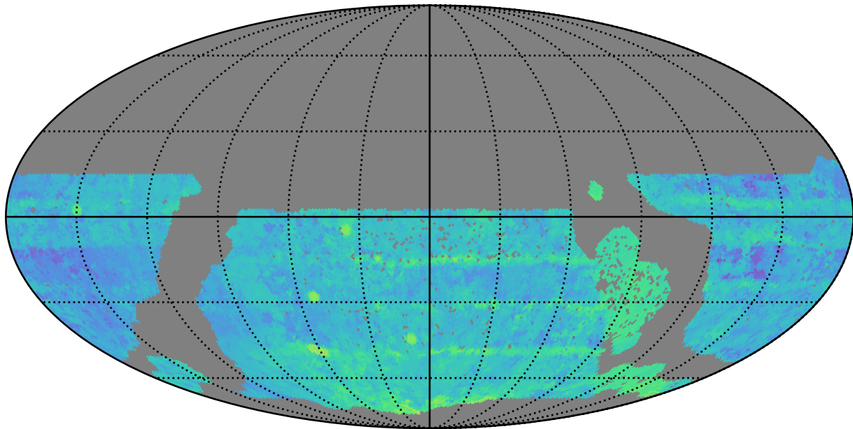
early_ss_template_fpextra2.0_v3.4_10yrs WFD r band: Median Season Length
