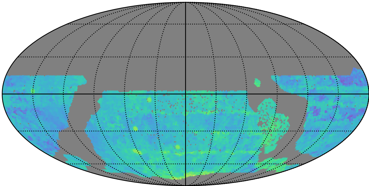
early_ss_template_fpextra2.0_v3.4_10yrs WFD i band: Median Season Length
