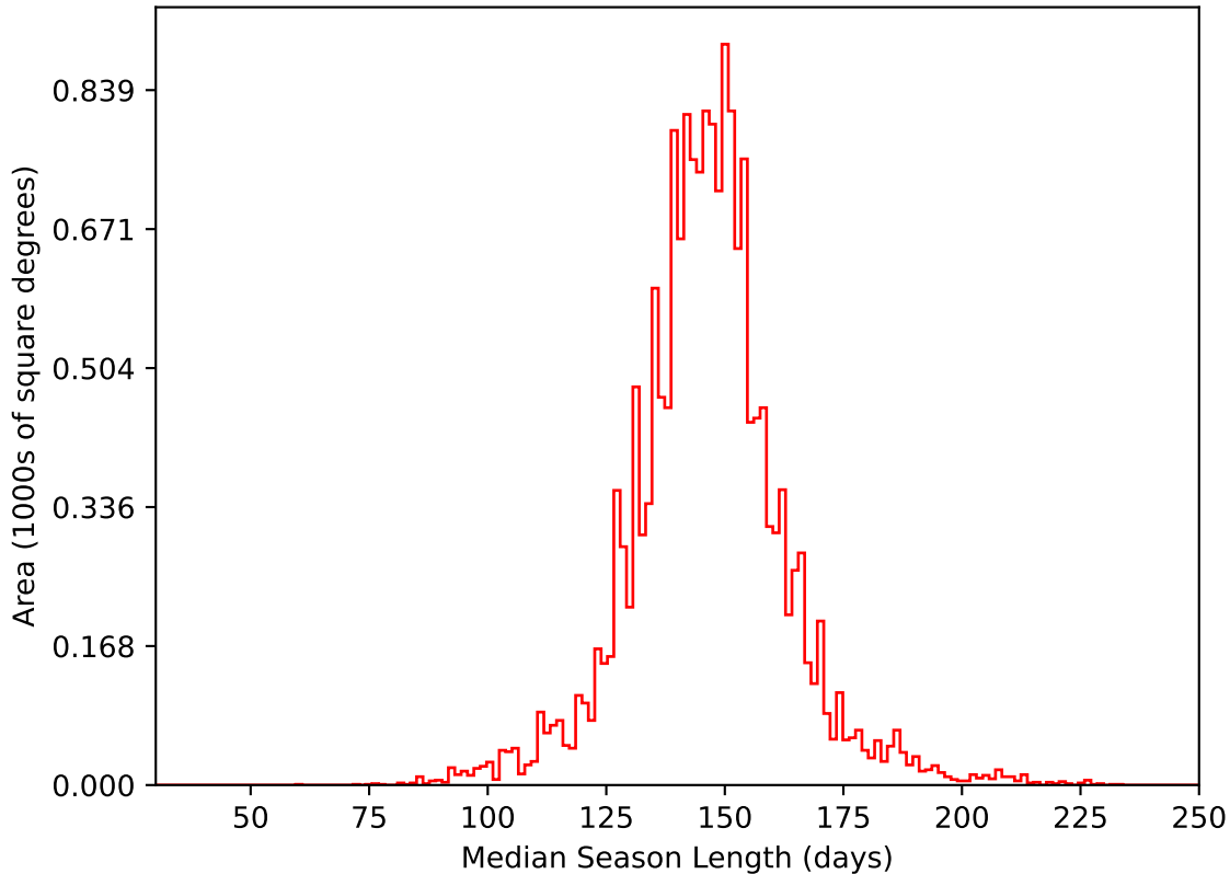
early_ss_template_fpextra2.0_v3.4_10yrs WFD i band: Median Season Length
