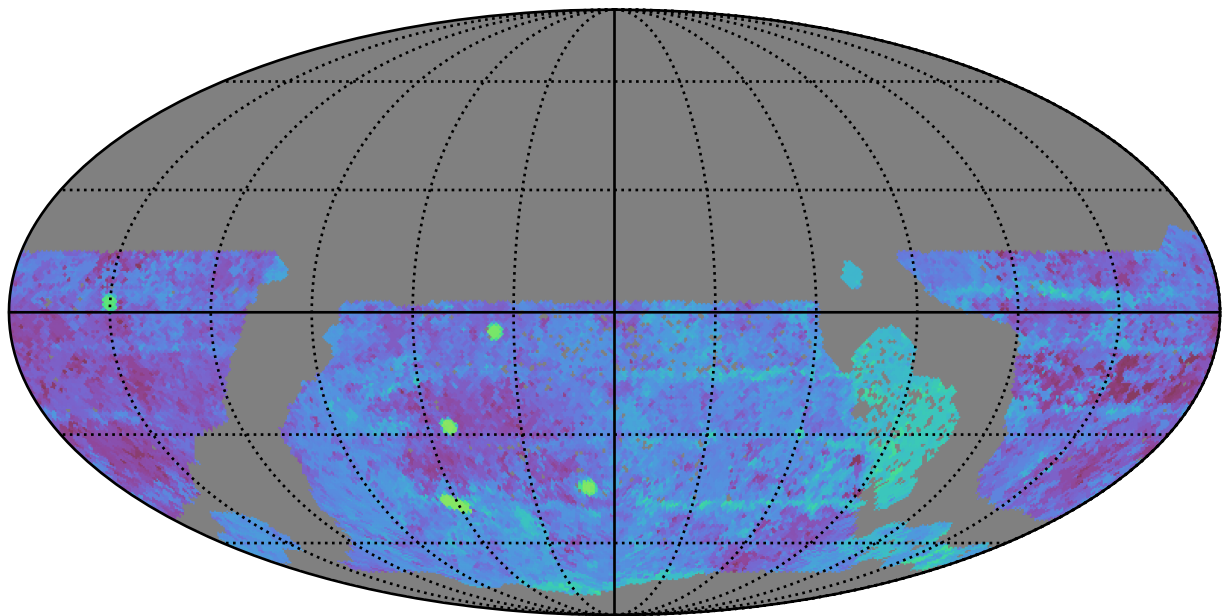
early_ss_template_fpextra2.0_v3.4_10yrs WFD g band: Median Season Length
