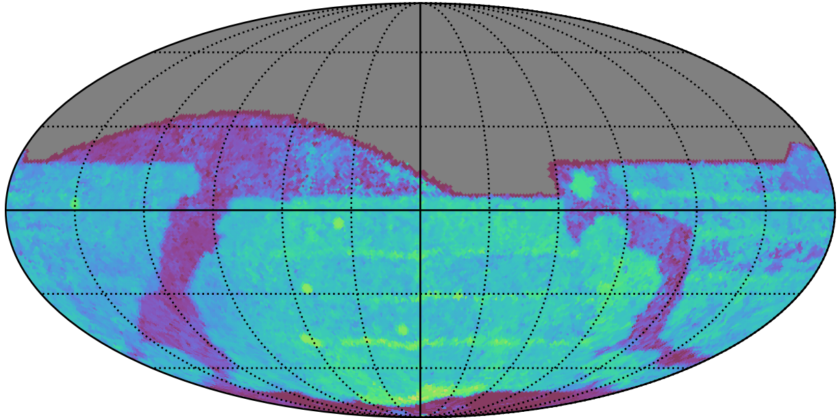
early_ss_template_fpextra2.0_v3.4_10yrs All sky z band: Median Season Length
