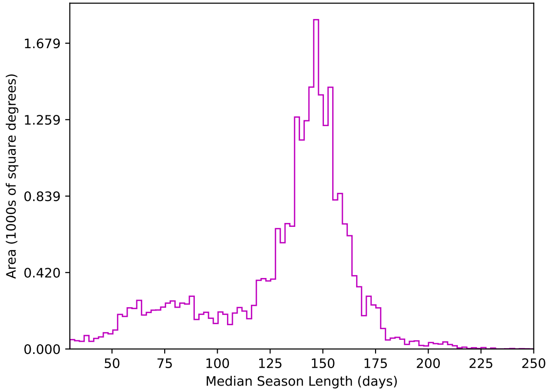
early_ss_template_fpextra2.0_v3.4_10yrs All sky z band: Median Season Length
