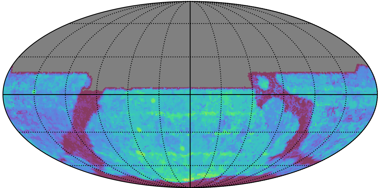
early_ss_template_fpextra2.0_v3.4_10yrs All sky y band: Median Season Length
