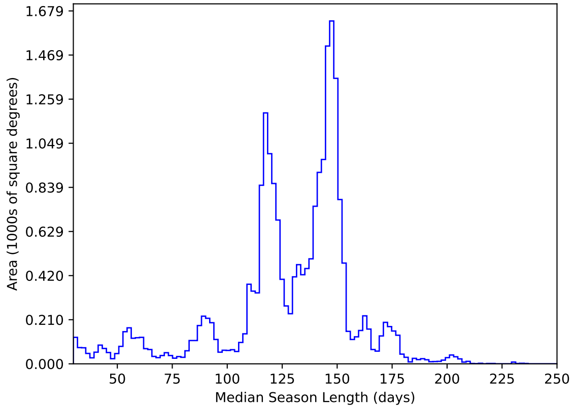
early_ss_template_fpextra2.0_v3.4_10yrs All sky y band: Median Season Length
