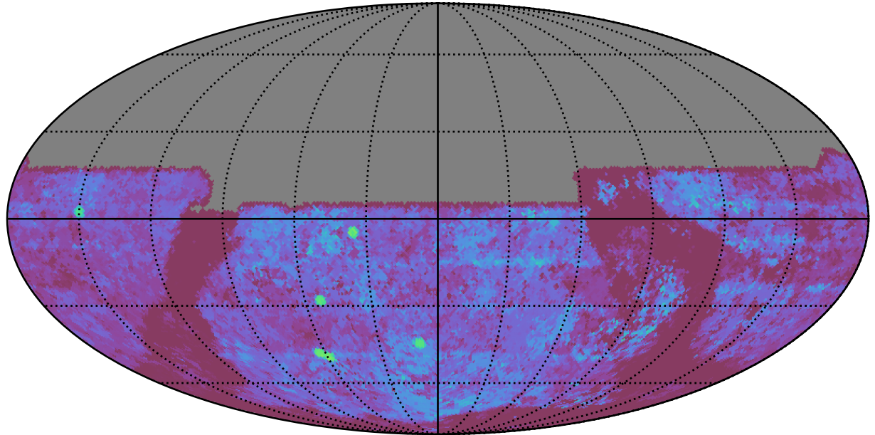
early_ss_template_fpextra2.0_v3.4_10yrs All sky u band: Median Season Length
