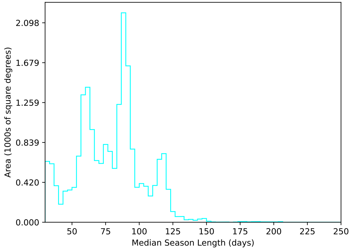
early_ss_template_fpextra2.0_v3.4_10yrs All sky u band: Median Season Length
