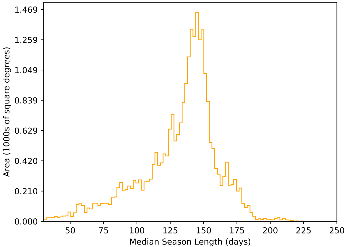
early_ss_template_fpextra2.0_v3.4_10yrs All sky r band: Median Season Length
