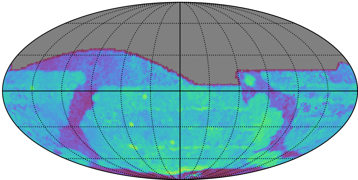
early_ss_template_fpextra2.0_v3.4_10yrs All sky i band: Median Season Length
