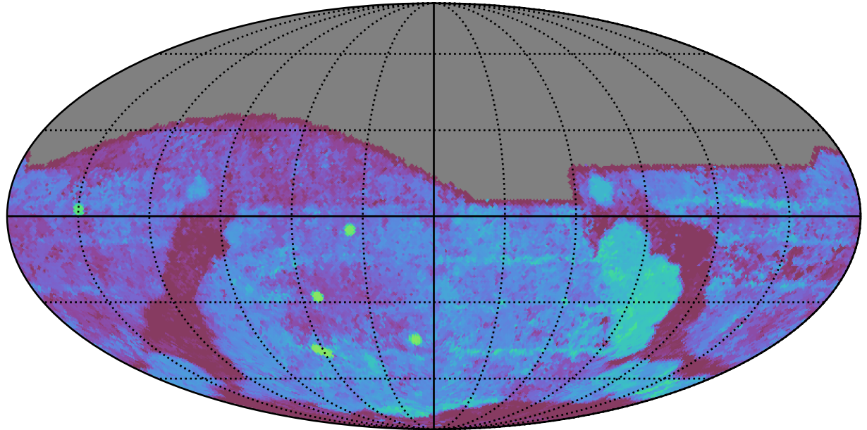
early_ss_template_fpextra2.0_v3.4_10yrs All sky g band: Median Season Length
