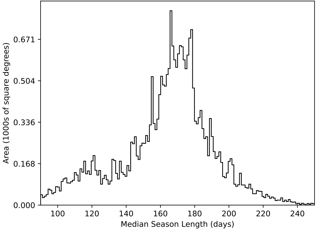
early_ss_template_fpextra2.0_v3.4_10yrs All sky all bands: Median Season Length
