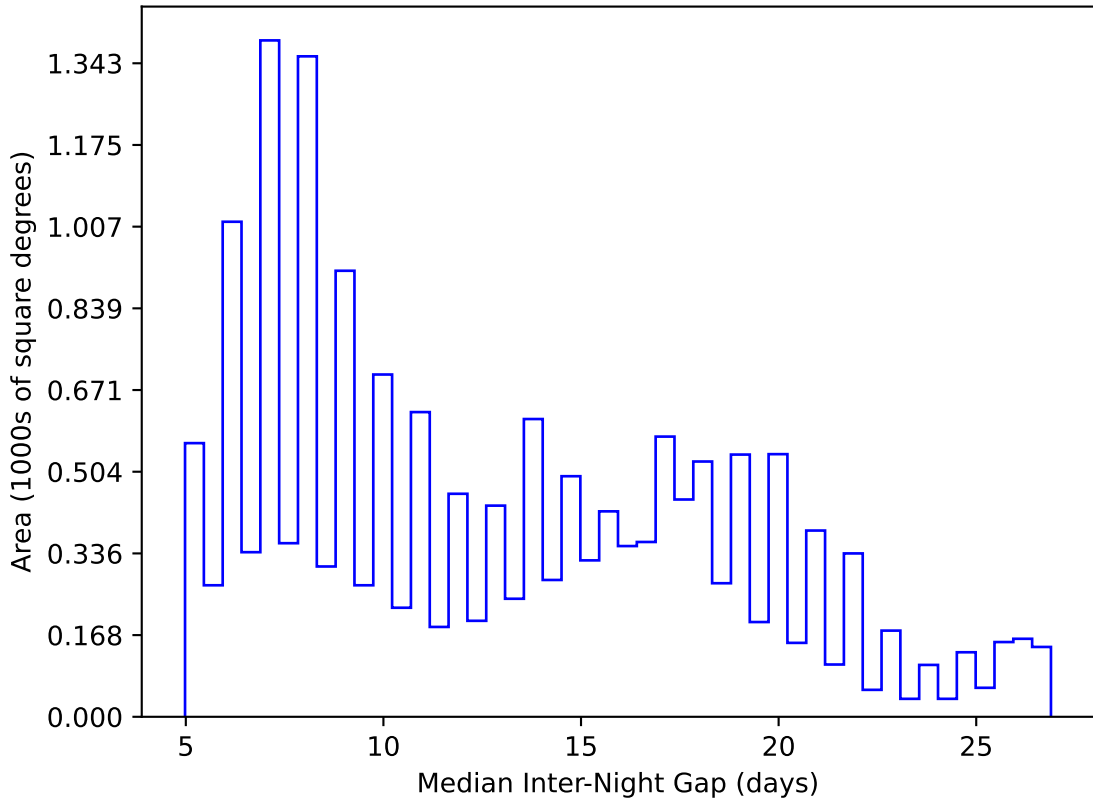
early_ss_template_fpextra2.0_v3.4_10yrs WFD y band: Median Inter-Night Gap
