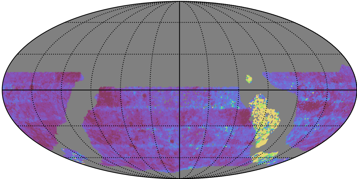
early_ss_template_fpextra2.0_v3.4_10yrs WFD u band: Median Inter-Night Gap
