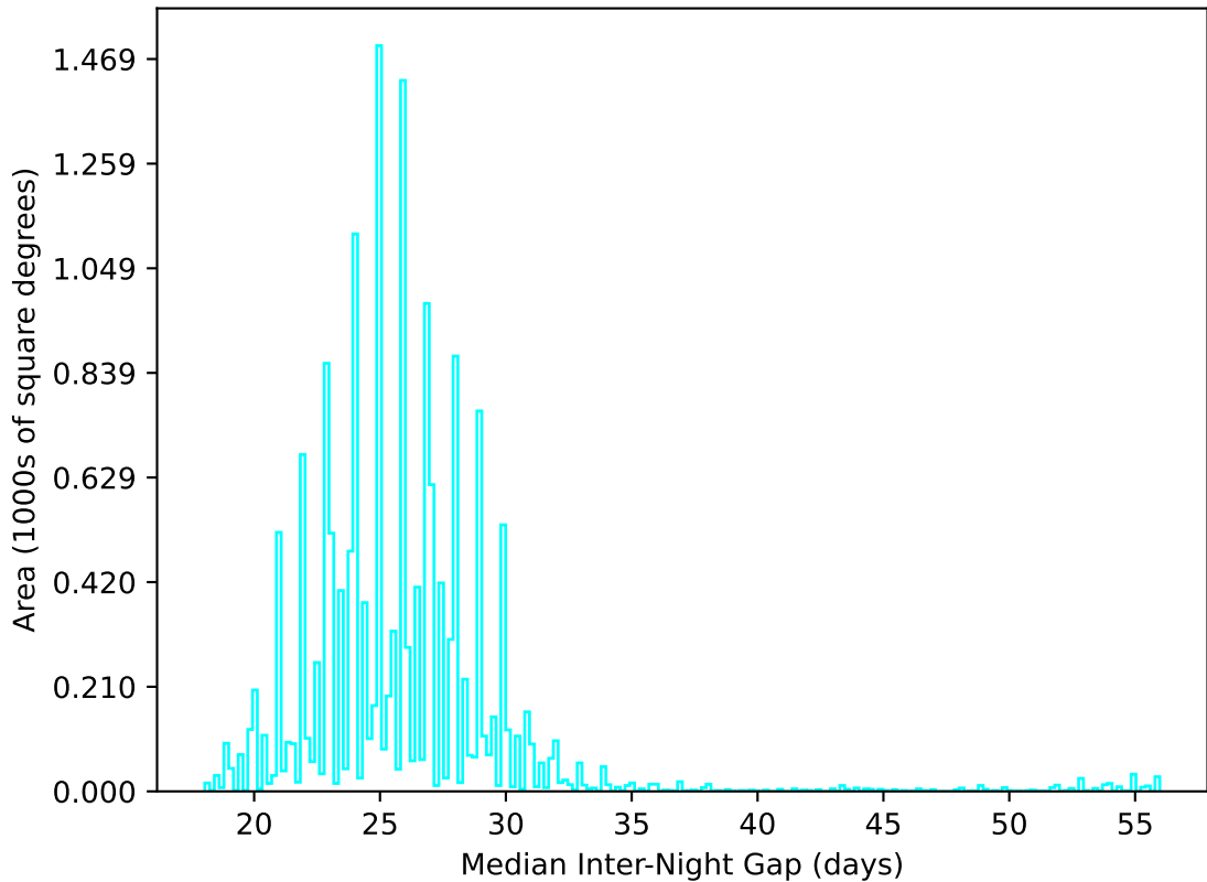
early_ss_template_fpextra2.0_v3.4_10yrs WFD u band: Median Inter-Night Gap
