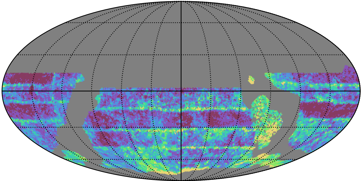
early_ss_template_fpextra2.0_v3.4_10yrs WFD r band: Median Inter-Night Gap
