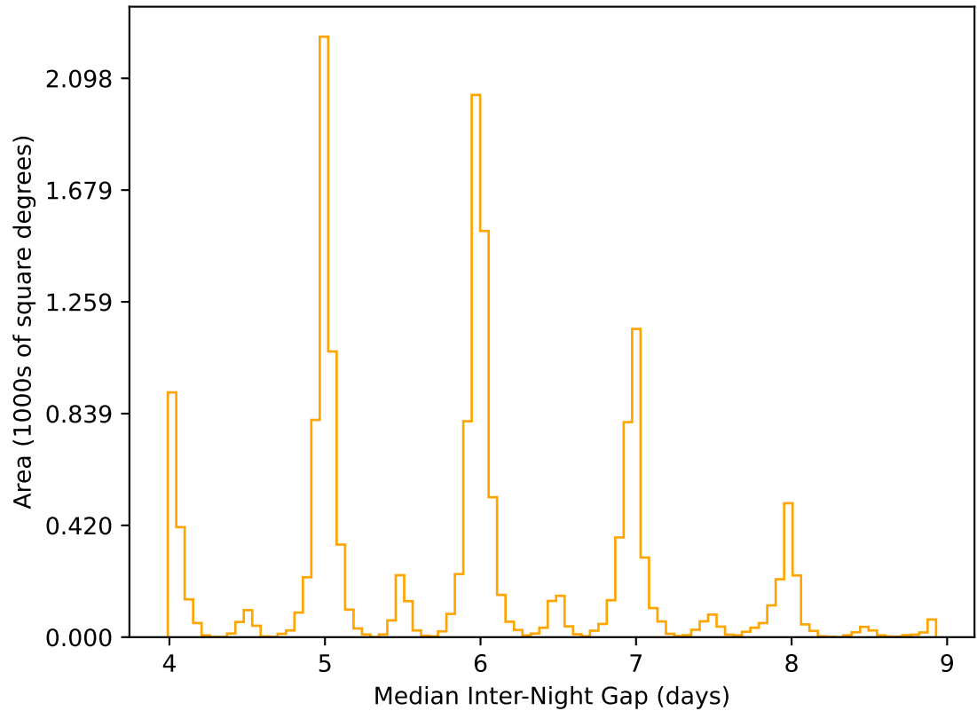
early_ss_template_fpextra2.0_v3.4_10yrs WFD r band: Median Inter-Night Gap
