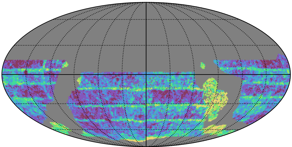
early_ss_template_fpextra2.0_v3.4_10yrs WFD i band: Median Inter-Night Gap
