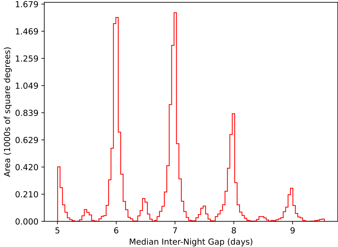
early_ss_template_fpextra2.0_v3.4_10yrs WFD i band: Median Inter-Night Gap
