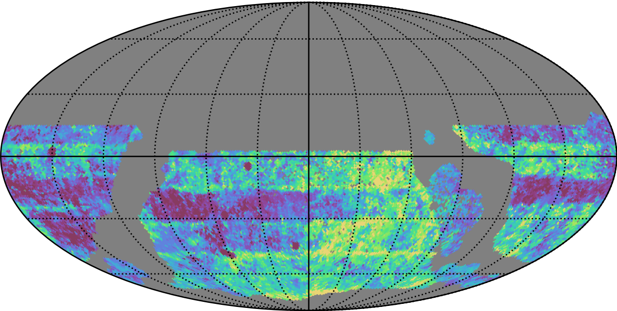
early_ss_template_fpextra2.0_v3.4_10yrs WFD g band: Median Inter-Night Gap
