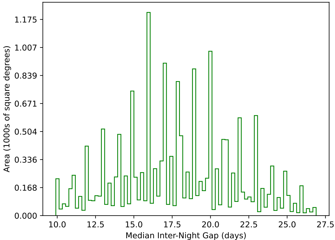
early_ss_template_fpextra2.0_v3.4_10yrs WFD g band: Median Inter-Night Gap
