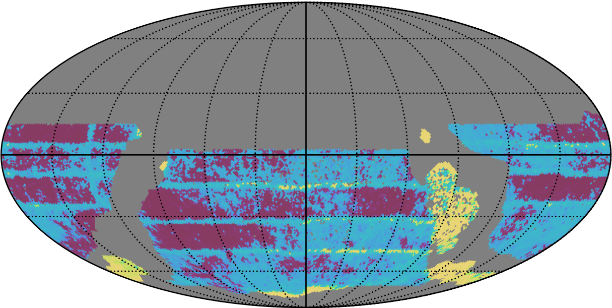
early_ss_template_fpextra2.0_v3.4_10yrs WFD all bands: Median Inter-Night Gap
