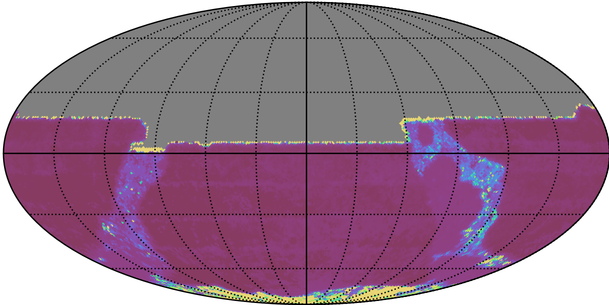
early_ss_template_fpextra2.0_v3.4_10yrs All sky y band: Median Inter-Night Gap
