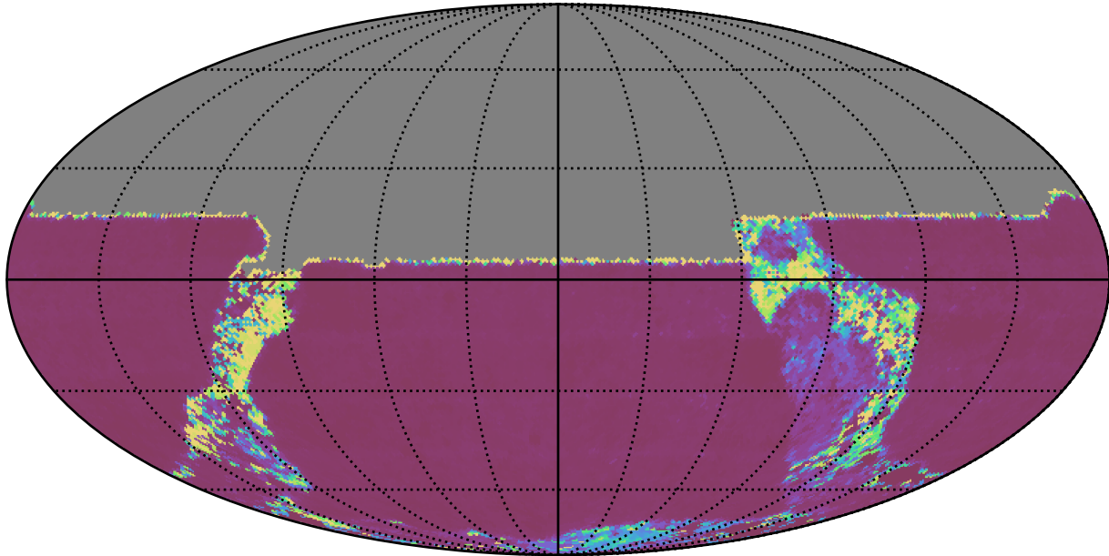
early_ss_template_fpextra2.0_v3.4_10yrs All sky u band: Median Inter-Night Gap
