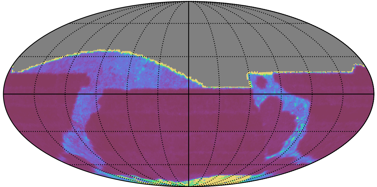
early_ss_template_fpextra2.0_v3.4_10yrs All sky r band: Median Inter-Night Gap
