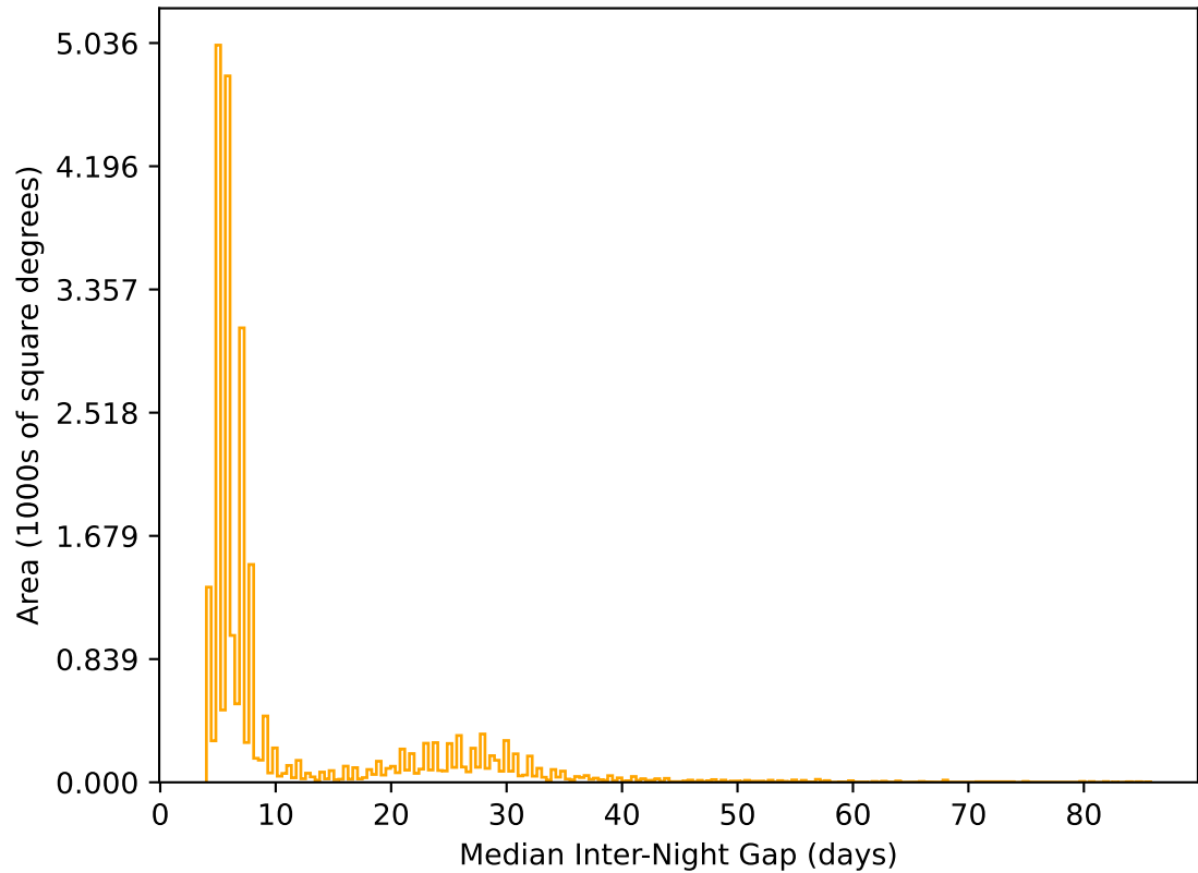
early_ss_template_fpextra2.0_v3.4_10yrs All sky r band: Median Inter-Night Gap
