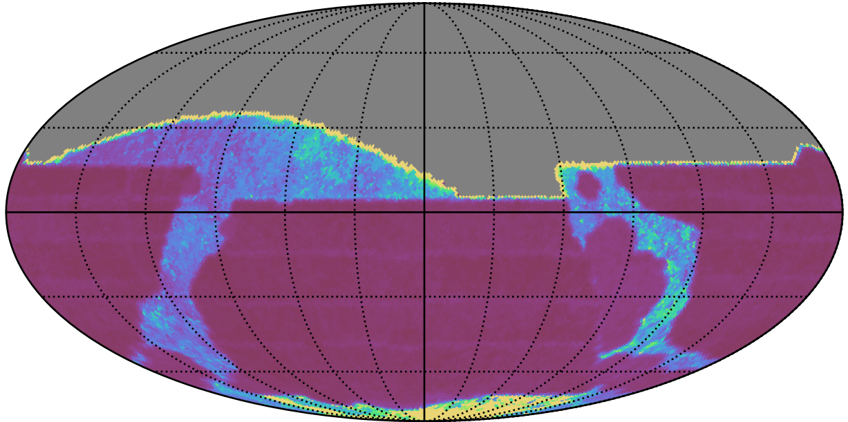
early_ss_template_fpextra2.0_v3.4_10yrs All sky i band: Median Inter-Night Gap
