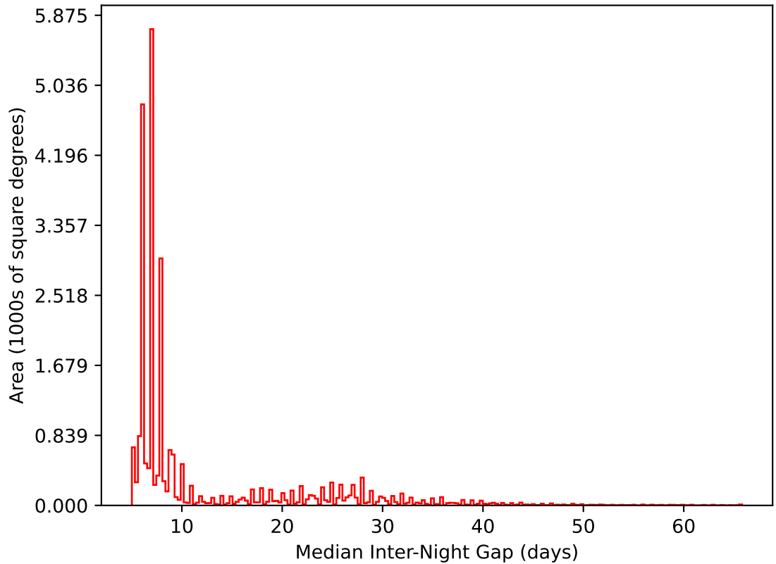
early_ss_template_fpextra2.0_v3.4_10yrs All sky i band: Median Inter-Night Gap
