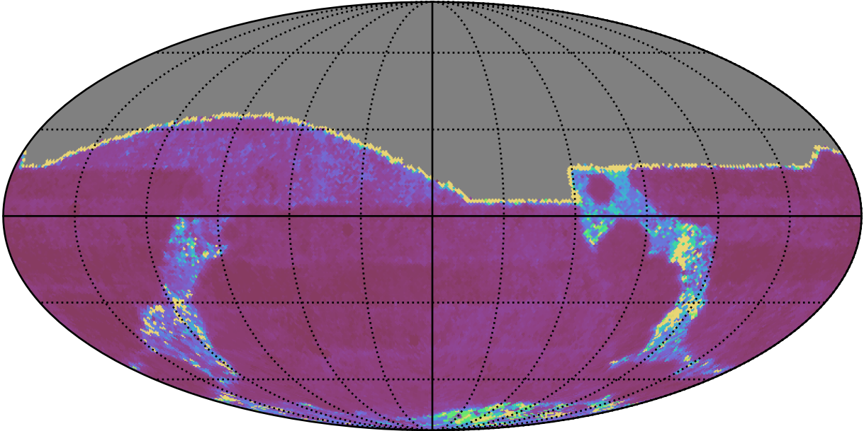
early_ss_template_fpextra2.0_v3.4_10yrs All sky g band: Median Inter-Night Gap
