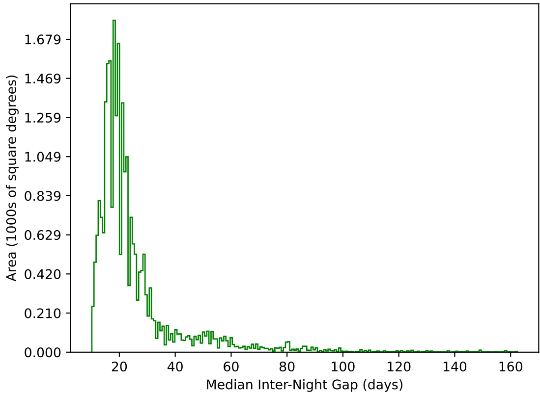
early_ss_template_fpextra2.0_v3.4_10yrs All sky g band: Median Inter-Night Gap
