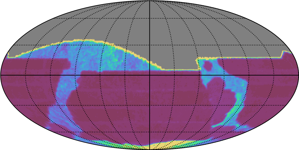
early_ss_template_fpextra2.0_v3.4_10yrs All sky all bands: Median Inter-Night Gap
