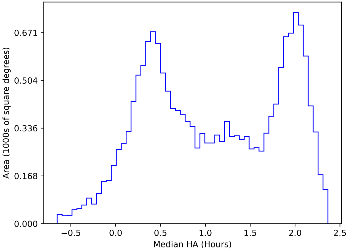
early_ss_template_fpextra2.0_v3.4_10yrs WFD z band: Median HA
