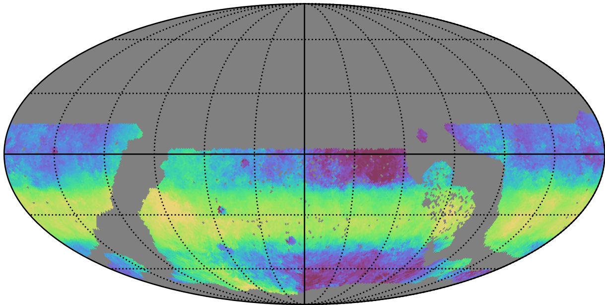
early_ss_template_fpextra2.0_v3.4_10yrs WFD y band: Median HA
