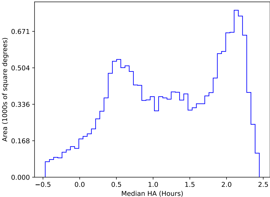
early_ss_template_fpextra2.0_v3.4_10yrs WFD y band: Median HA
