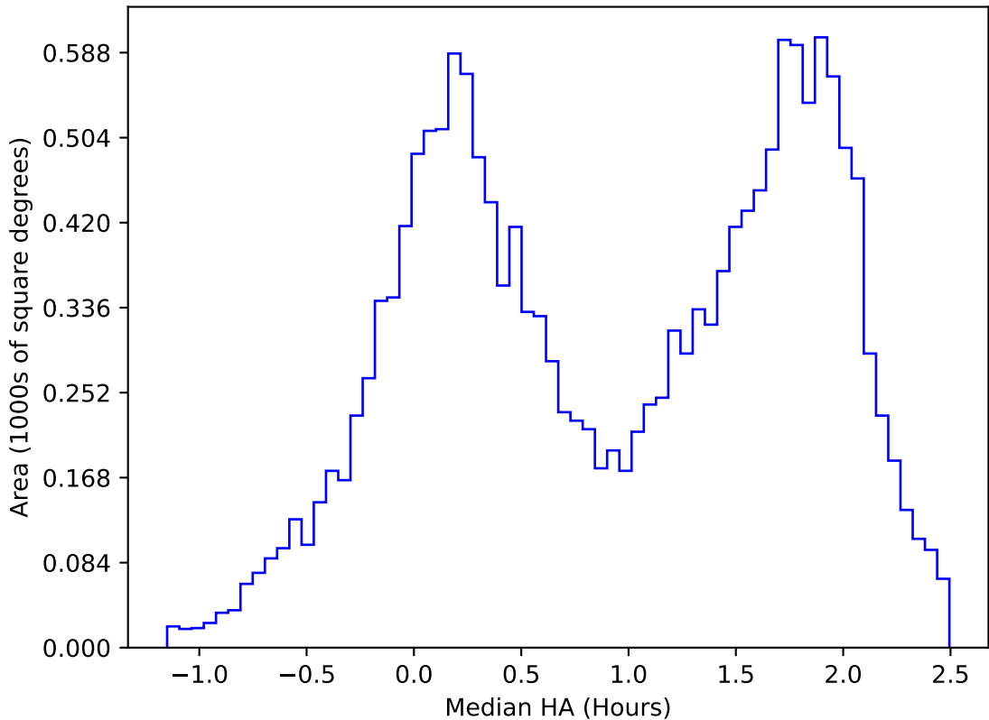
early_ss_template_fpextra2.0_v3.4_10yrs WFD u band: Median HA
