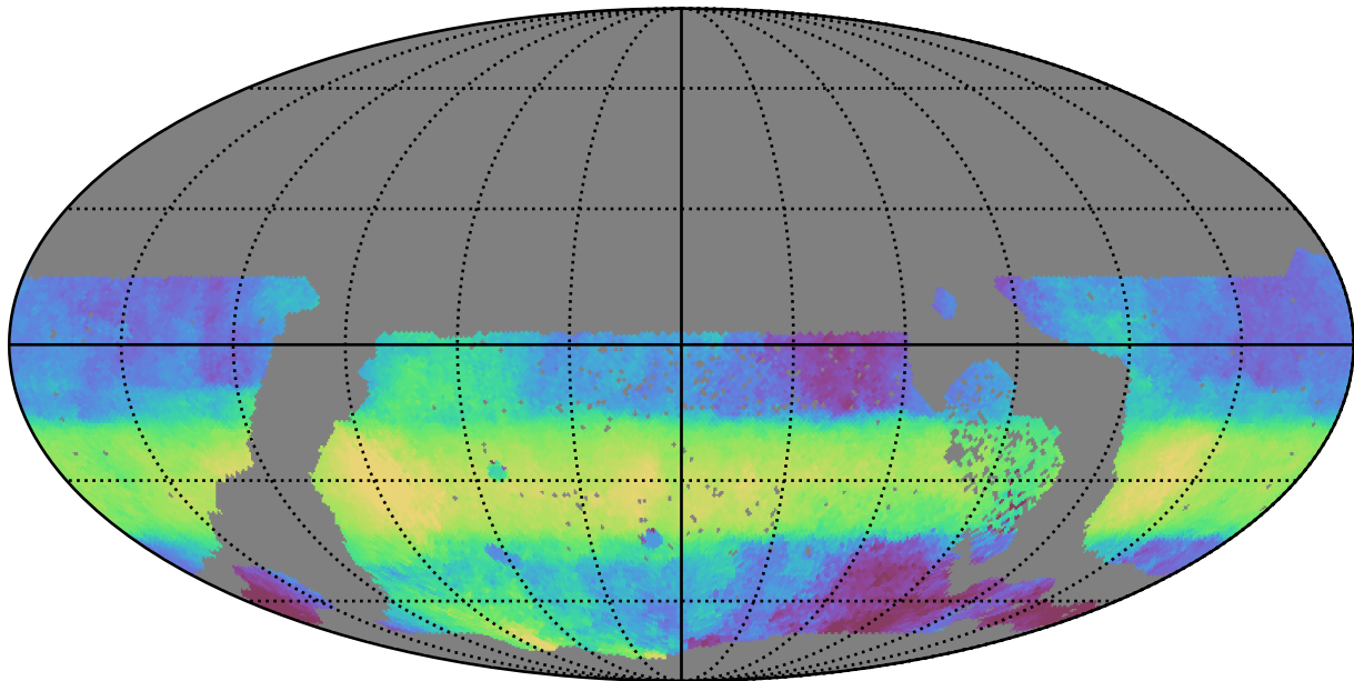
early_ss_template_fpextra2.0_v3.4_10yrs WFD r band: Median HA
